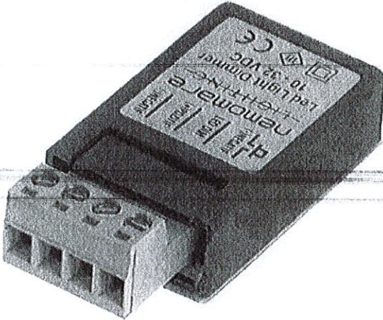
3.40 - 24 volt dc led dimmer ( 10 – 32 vdc)
